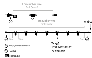
498 EC-MAIN-1-7-B Cable 1m - 7 connectors black 498 EC-MAIN-1-7-W Cable 1m - 7 connectors white
