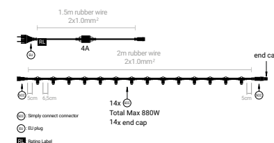
498 EC-MAIN-2-14-B Cable 2m - 14 connectors black 498 EC-MAIN-2-14-W Cable 2m - 14 connectors white
