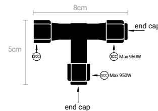
498 EC-T-B T connector black 498 EC-T-W T connector white
