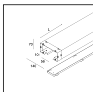
100652.99 Housing box L=1125mm.
